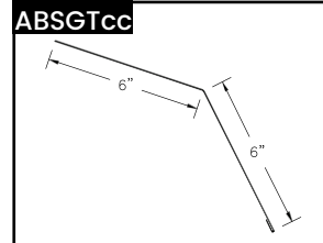
ABS Gambrel Trim
