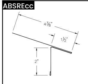
ABS Residential Eave
