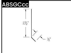
ABS Gable Cleat
