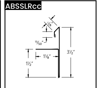
ABS Slim Line Rake
