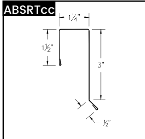
ABS Rake Trim
