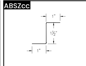
ABS Metal "Z" Closure
