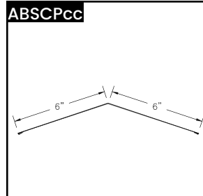
ABS 6" Ridge Cap
