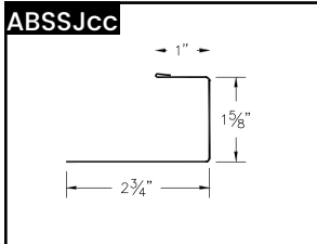
ABS Starter "J"
