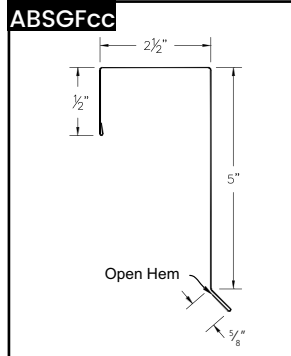
ABS Gable Flasing
