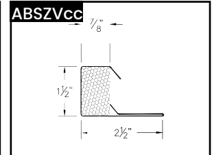
ABS Vented "Z" Closure
