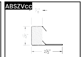
ABS Vented "Z" Closure
