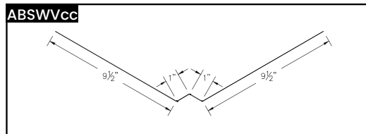
ABS W Valley
