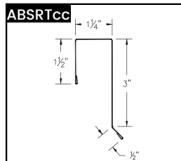
ABS Rake Trim
