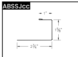
ABS Starter "J"
