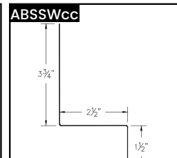
ABS Sidewall
