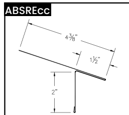
ABS Residential Eave
