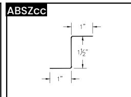
ABS Metal "Z" Closure
