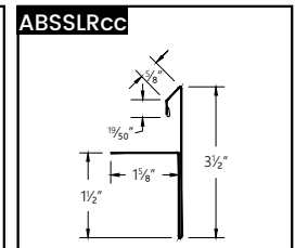
ABS Slim Line Rake
