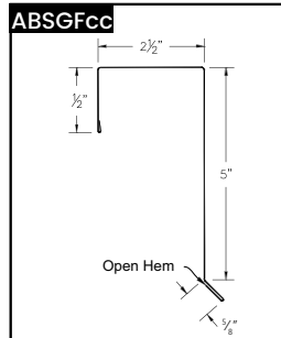
ABS Gable Flasing
